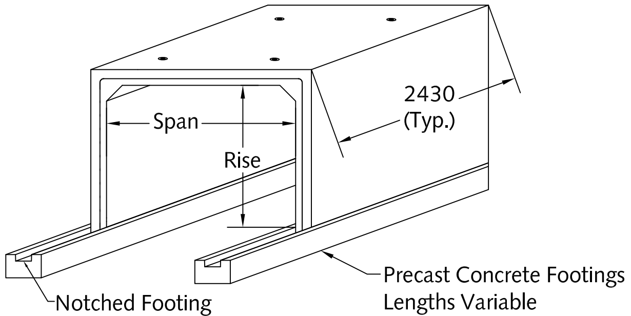
Isometric View
