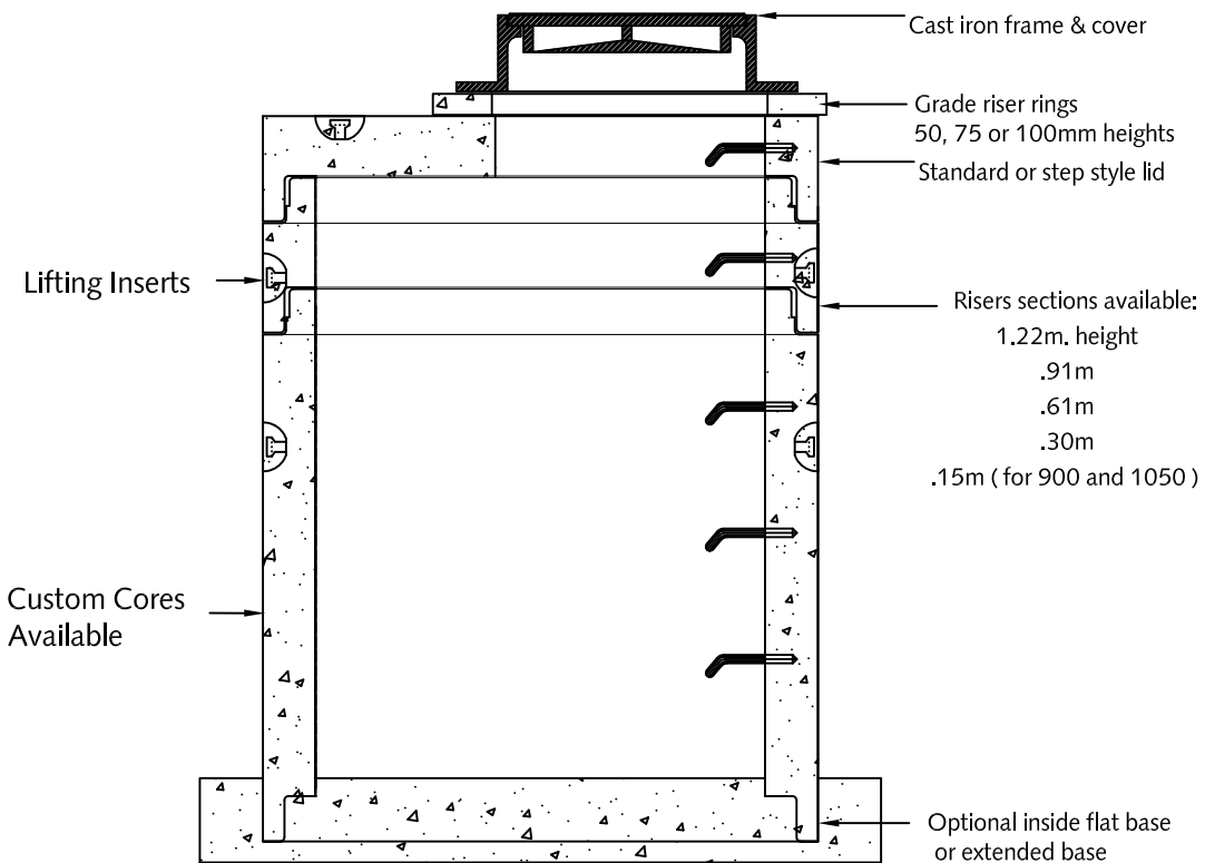
Section View of Typical Manhole
