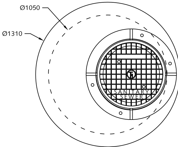
Plan View of Manhole w/Lid and Cover
