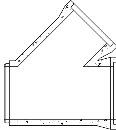
Concrete Wye Off
