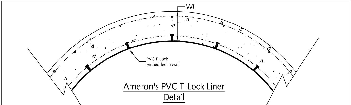
Section View
