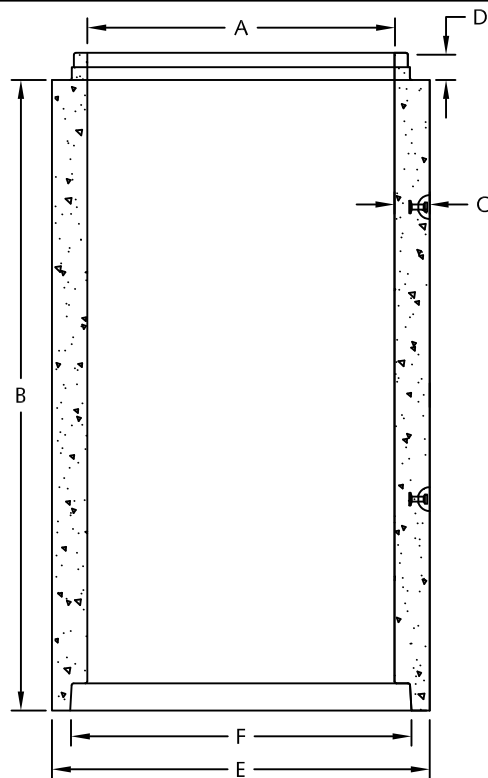
Straight Wall-Tongue & Groove Pipe (1050-1800 mm)
