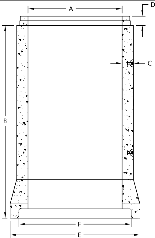
Bell & Spigot Pipe (300-900 mm)
