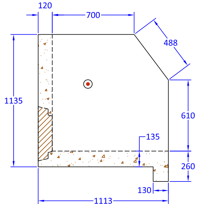
Wing Wall Detail
