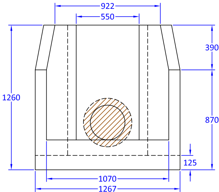
Elevation View
