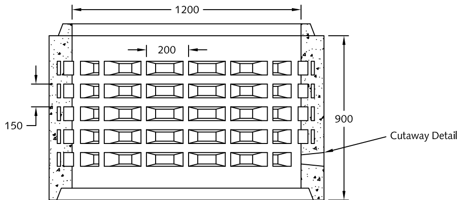
Section View of Ø1200 Drywell Barrel
