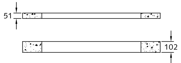
TR36/TRC1 Frame
