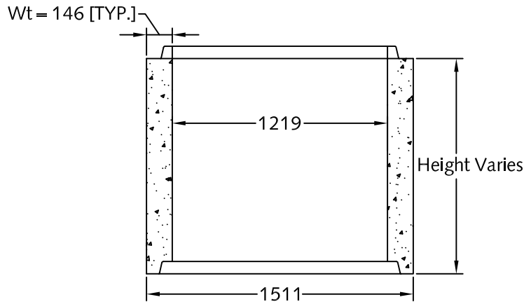
Section View
