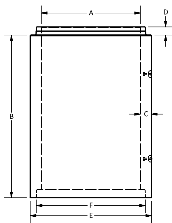
Straight Wall - Tongue & Groove Pipe (1050 - 1800 mm)
