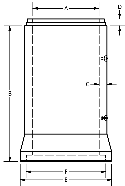
Bell & Spigot Pipe (300 - 900 mm)
