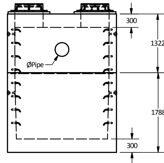
East View
