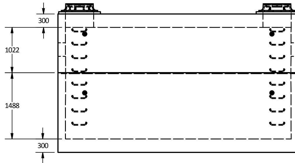
Elevation View
