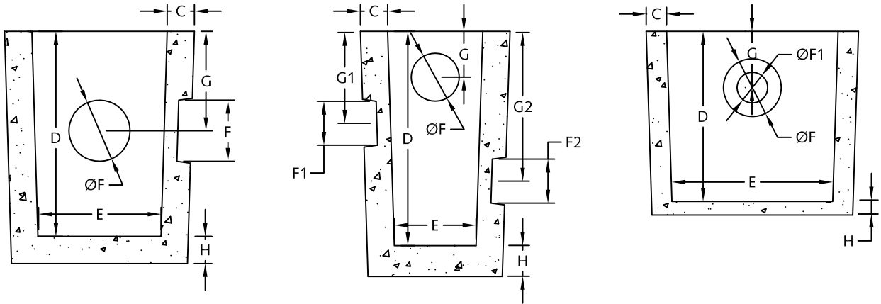
Elevation Views
