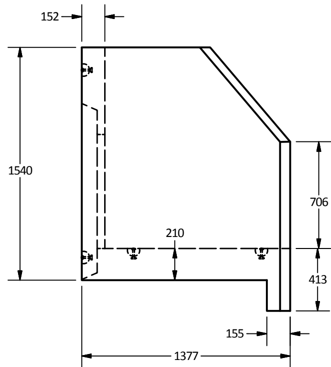
Side View
