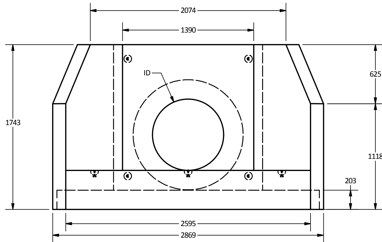
Elevation View
