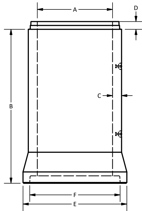
Bell & Spigot Pipe (200 - 1200mm)
