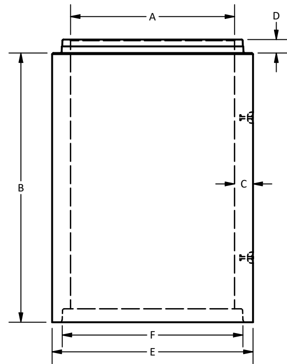
Straight Wall - Tongue & Groove Pipe (1350 - 3050 mm)
