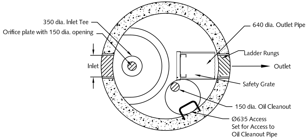
Plan View w/Pipe Orientation
