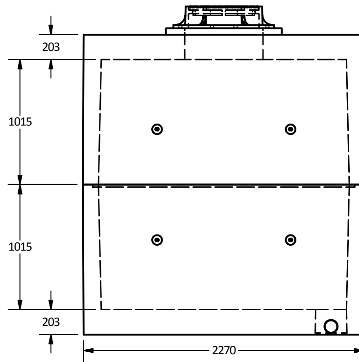
Elevation View
